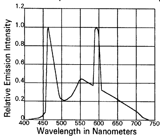
Emission Spectrum Combined White Full Spectrum and Amber LED Light Sources
