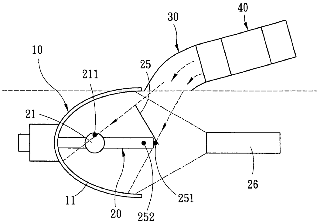
Fig.3 PRIOR ART
