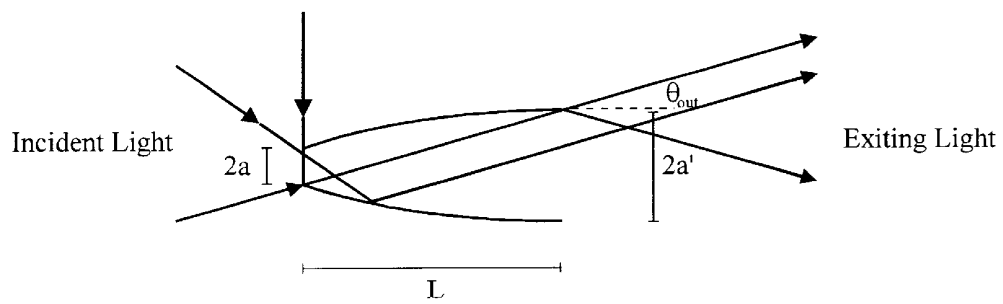
PRIOR ART Figure 11
