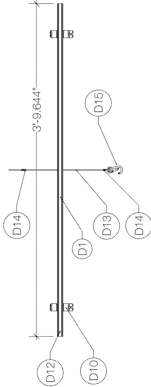
Fig. 26 Truss Mount Prototype Extrusion Top View Scale: 1 1/2" = 1'-0"
